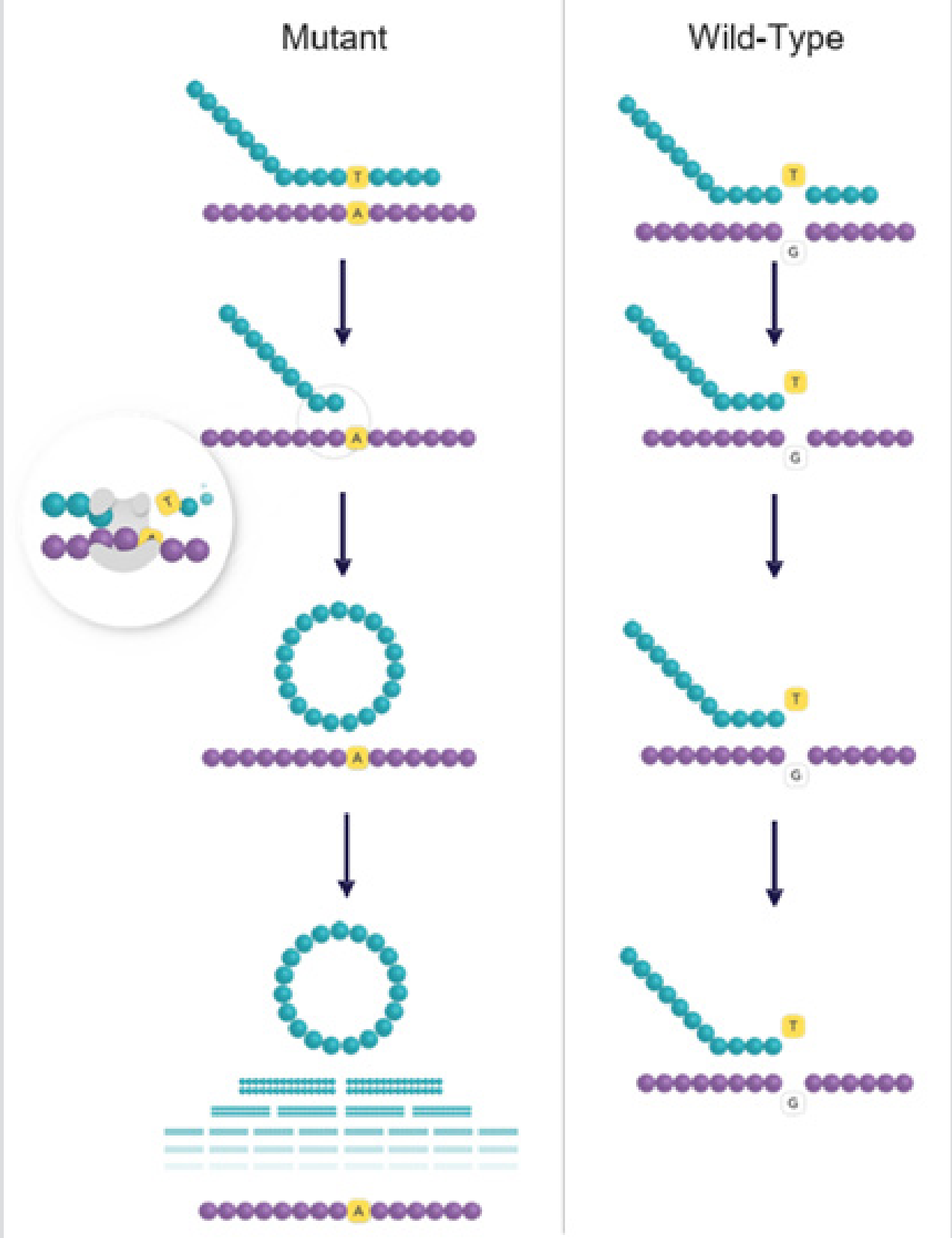
Figure 2: Aspyre technology. Aspyre probes hybridize to both wild-type (WT) and mutant (MT) DNA but are mismatched to WT molecules. Reverse polymerization specifically digests only perfectly matched probes annealed to mutated DNA. Those annealed to WT DNA are not digested due to mismatch. Digested probes from MT DNA are released and circularized by ligation, while the non-digested probes remain double stranded to WT DNA. Circularized probes from MT DNA are isothermally amplified and detected using fluorescent dye(s). Probes that hybridized to WT molecules are not amplified.
